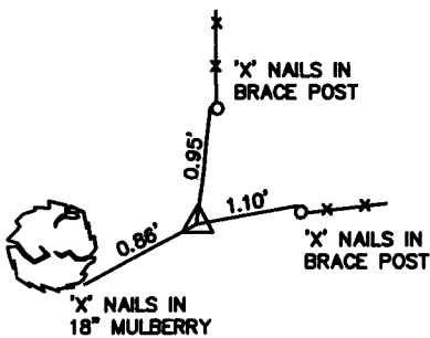
WEST QUARTER CORNER SEC. 25-T77N-R26W 1/2" IRON ROD WITH CAP #6808 (EXPOSED)
