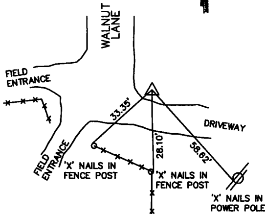
CENTER OF SECTION SEC. 25-T77N-R26W 1/2" IRON ROD WITH CAP #6808 (6" DEEP)
