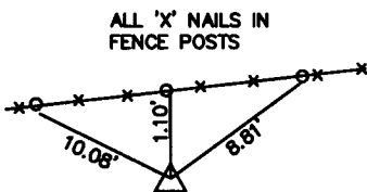
NORTHEAST CORNER OF THE NW 1/4 OF THE SW 1/4 SEC. 25-T77N-R26W 5/8" IRON ROD WITH CAP #14074 (EXPOSED)
