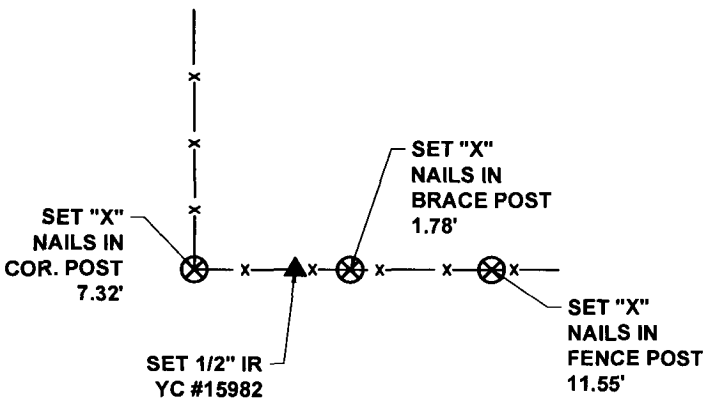
SW CORNER NW 1/4 NW 1/4 SECTION 26, TOWNSHIP 75 NORTH, RANGE 27 WEST
