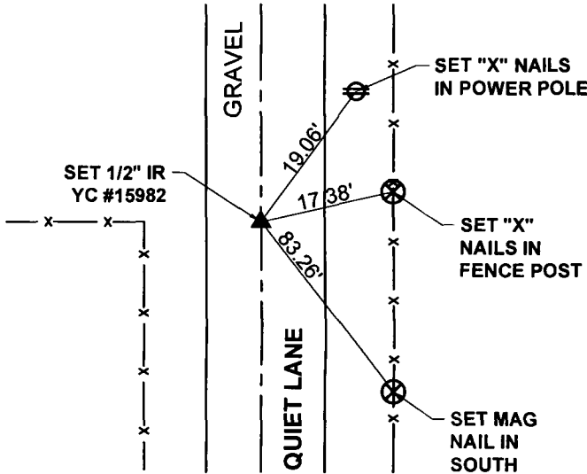
SE CORNER NW 1/4 NW 1/4 SECTION 26, TOWNSHIP 75 NORTH, RANGE 27 WEST
