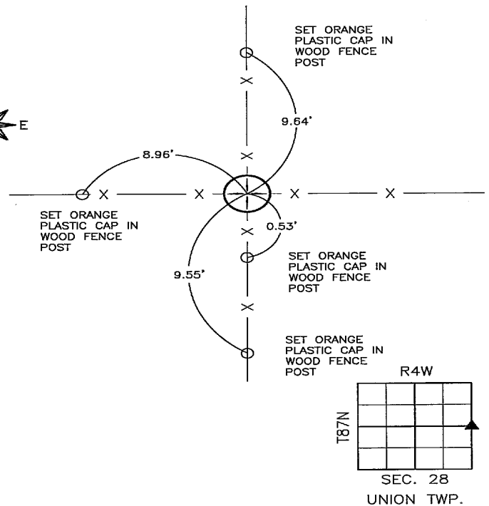
(2) E1/4 CORNER OF SEC. 28-87-4
