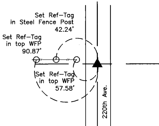
W 1/4 Corner Set 1/2"Ø Rebar w/ Orange Plastic Cap PLS 17939
