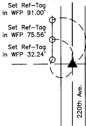
SW Corner NW 1/4-SW 1/4 Set 1/2"Ø Rebar w/ Orange Plastic Cap PLS 17939
