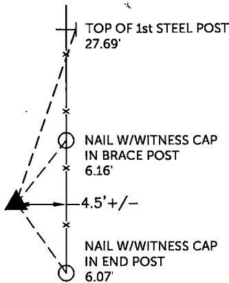
CENTER OF SECTION SET 1/2" REBAR W/ORANGE CAP #17939
