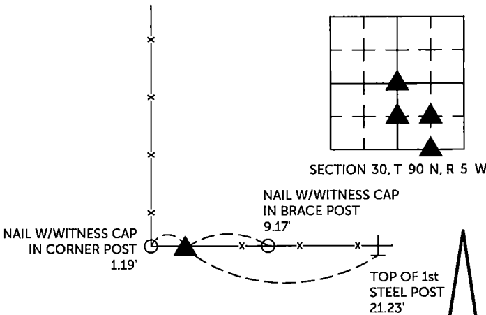
NW CORNER SW 1/4 - SE 1/4 SET 1/2" REBAR W/ORANGE CAP #17939
