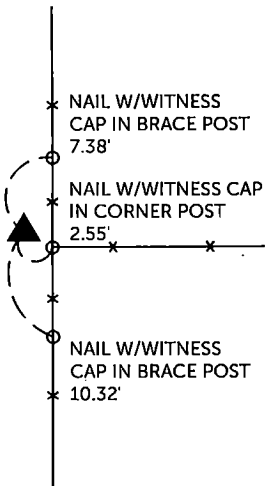
NW CORNER SW 1/4 - SE 1/4 SET 1/2" REBAR W/ORANGE CAP #17939
